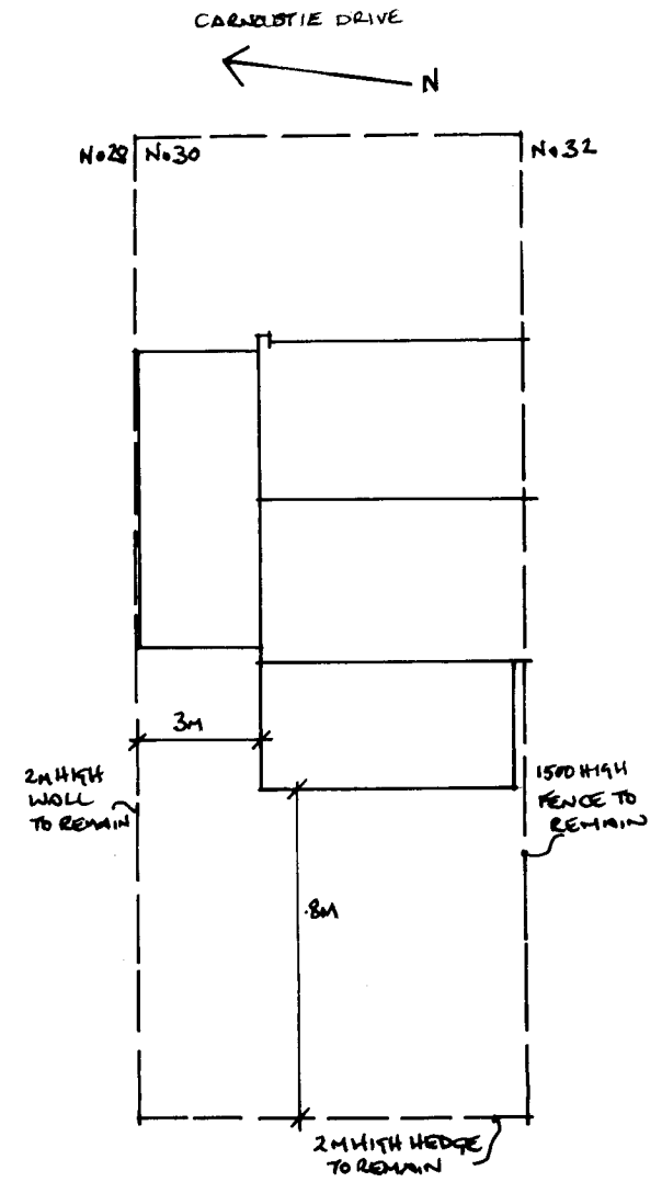
PROPOSED SITE AND ROOF PLAN 1:200
